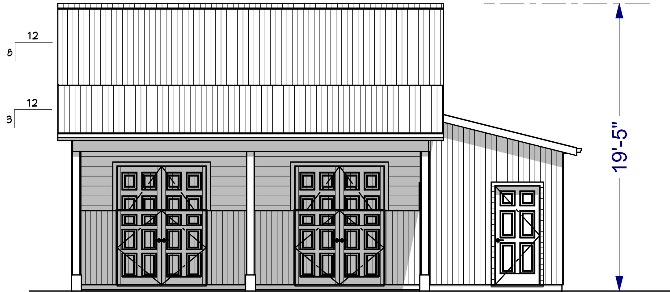
FRONT ELEVATION
