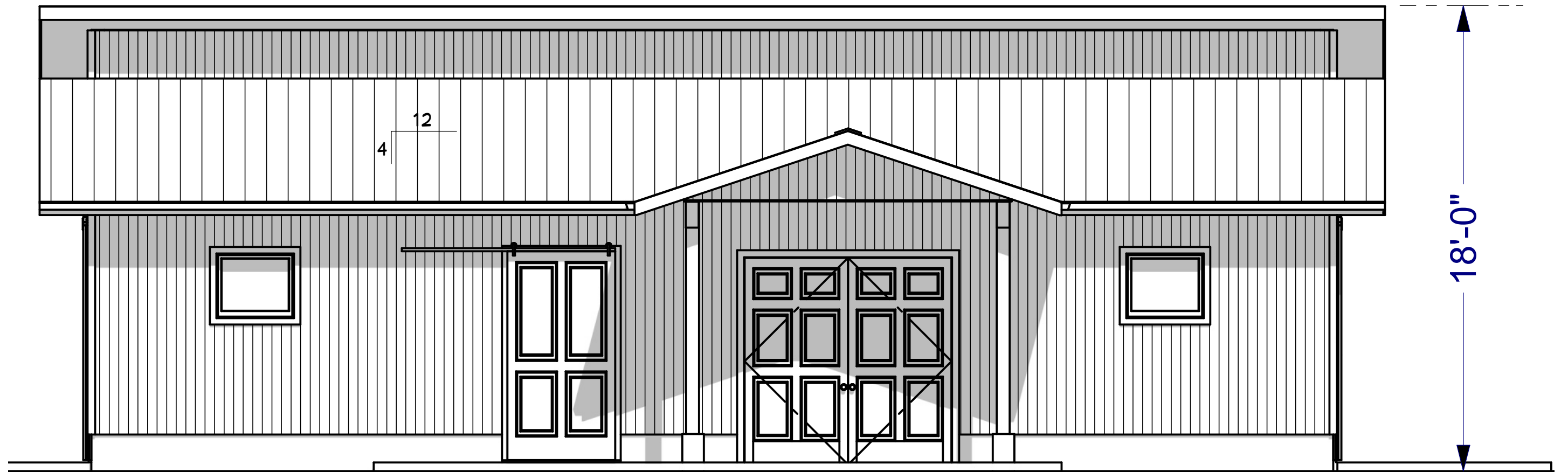
FRONT ELEVATION
