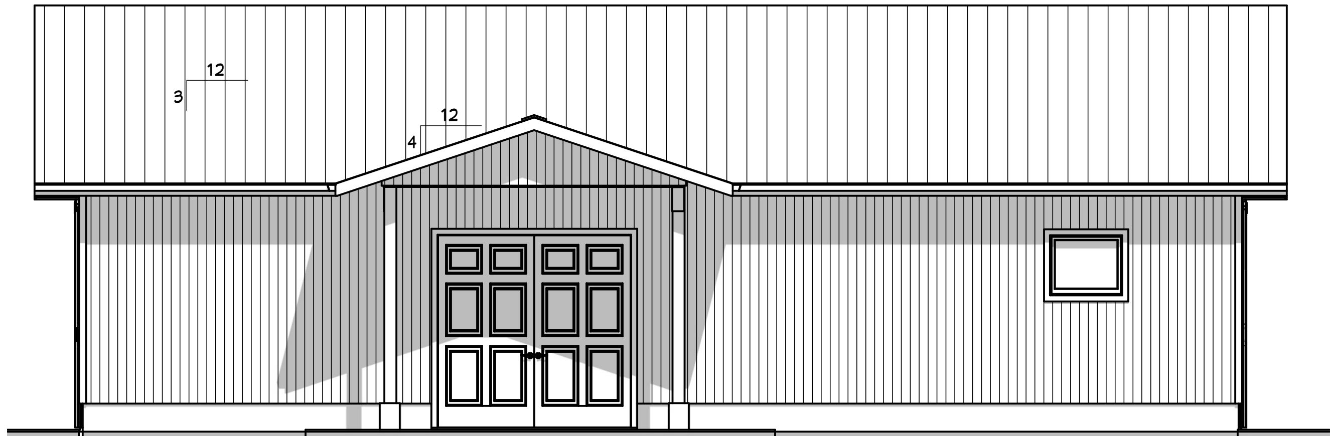
REAR ELEVATION
